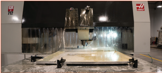
GR-712: 8100 RPM spindle: (X145" Y85" Z11") GR-510: 5000 RPM spindle: (X120" Y60" Z7.5")
